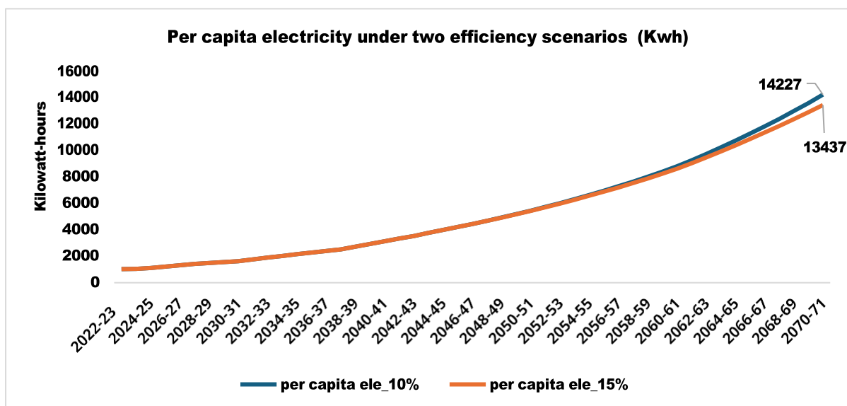
Figure 34: Per capita electricity consumption by 2070 across scenarios
