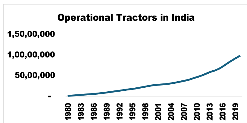
Figure 30: Demand for tractors in India
